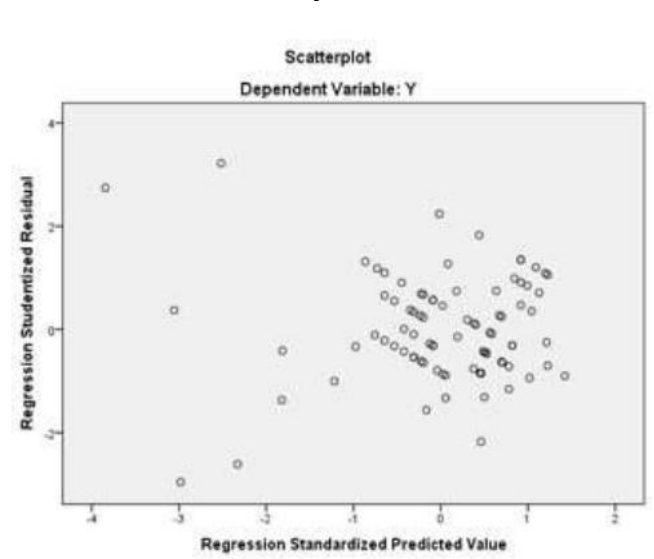
Picture 1 Heteroscedasititsity Test Result
